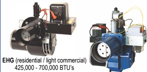
HSG 200/400 (residential) 60,000 - 400,000 BTU's
