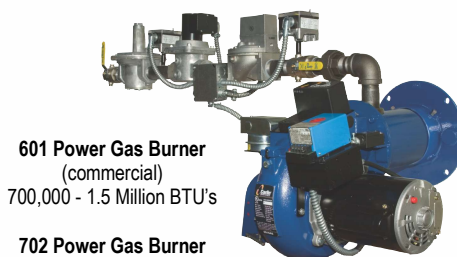
702 Power Gas Burner (commercial) 950,000 - 1.6 Million BTU's
