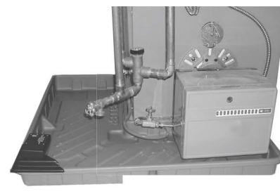
L-Shaped Burner Trays for Burner, Filter & Connections
