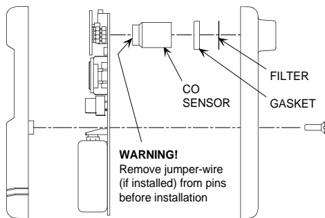
Figure 4. Sensor Installation
