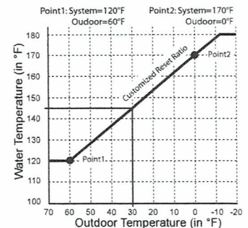
Custom Reset Ratio
