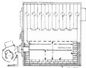
Brick combustion chamber, side view.
