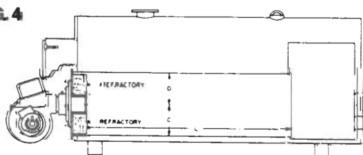
Scotch Marine boiler. No combustion chamber.
